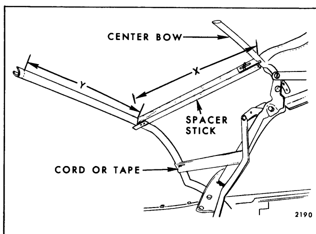
Fig. 13-46—Marking Back Curtain
