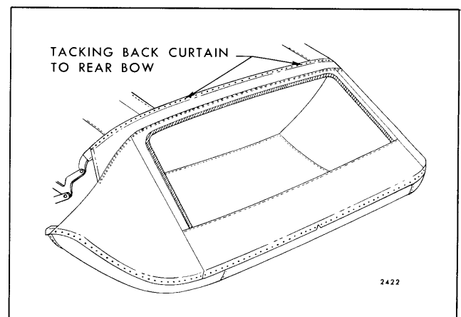
Fig. 13-16—Back Curtain Installed
