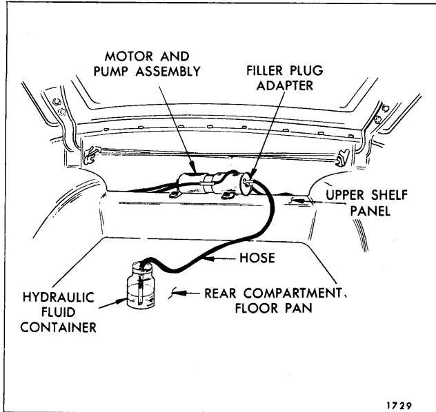
Fig. 13-68—Filling Reservoir
