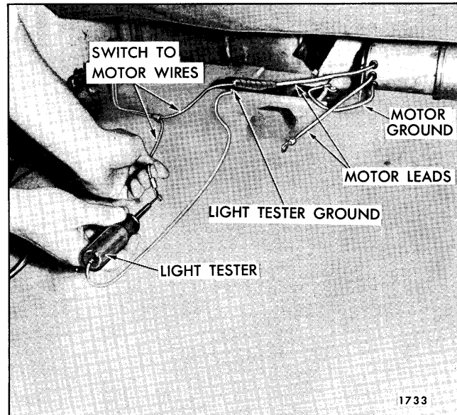
Fig. 13-63—Checking Motor Wiring
