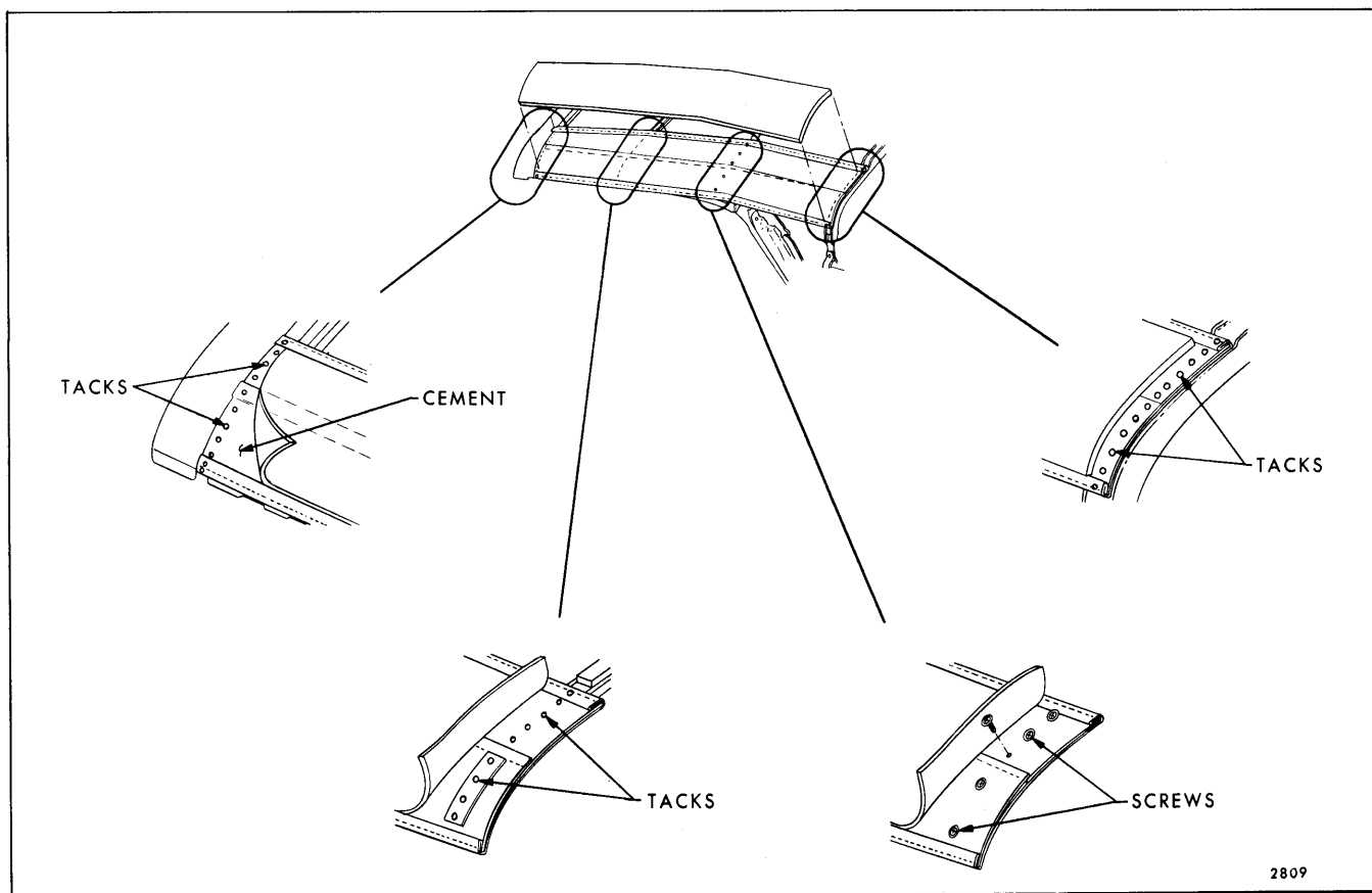
Fig. 13-12—Typical Side Stay Pad Installation
