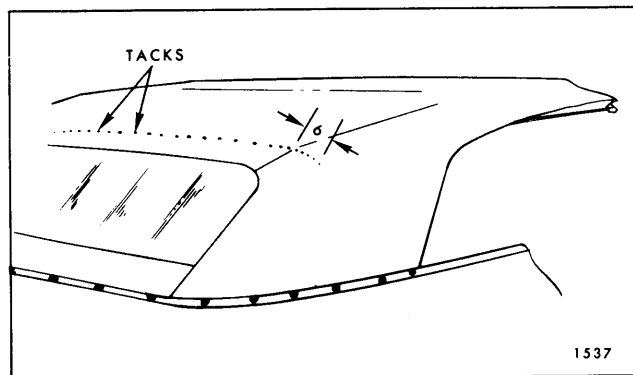
Fig. 13-38—Tacking Outboard of Seams
