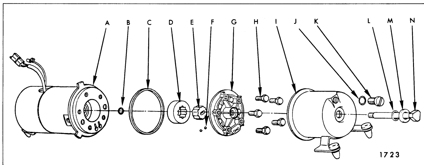
Fig. 13-56—Hydro-Lectric Motor And Pump Disassembled
