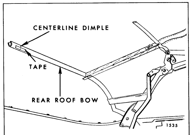
Fig. 13-20—Marking Rear Roof Bow
