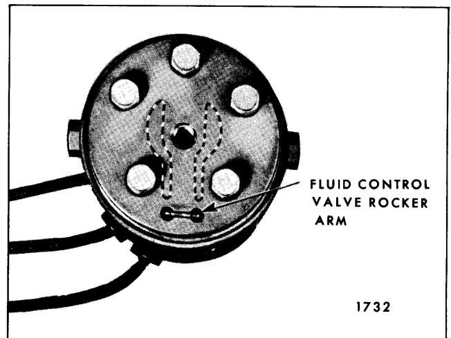
Fig. 13-60—Pump Cover Plate
