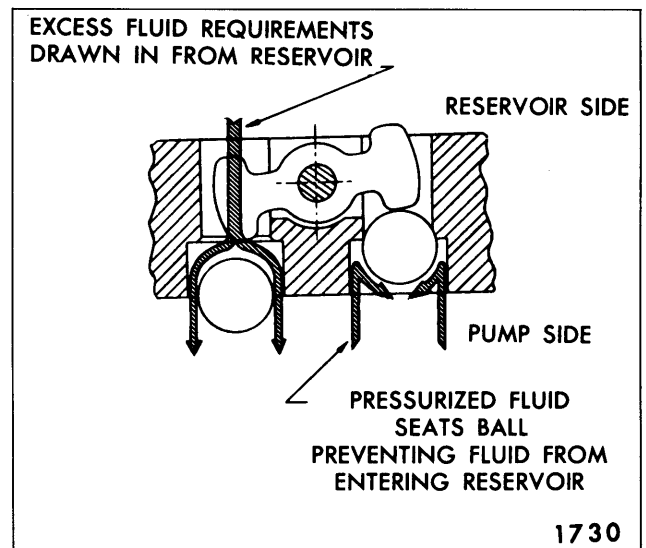
Fig. 13-61—Fluid Control Valve
