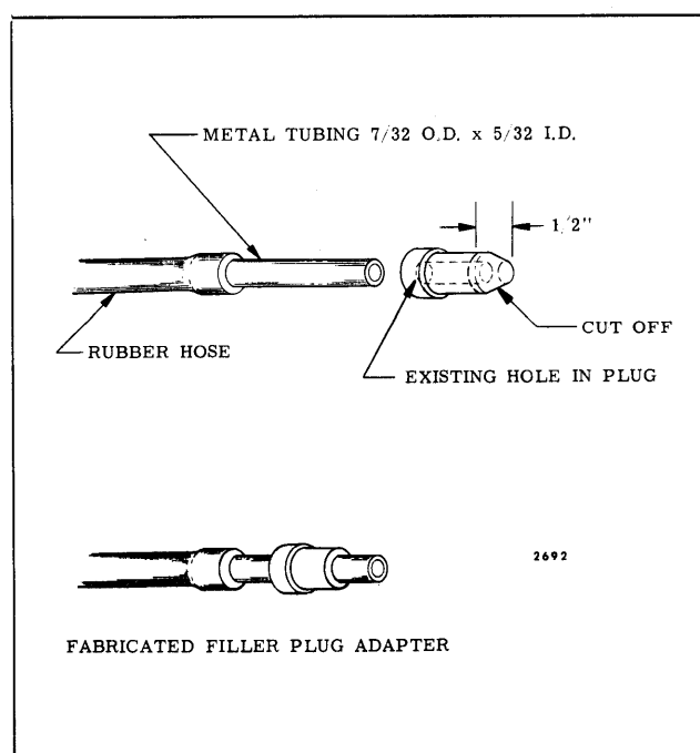
Fig. 13-67—Reservoir Filler Plug Adapter
