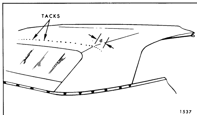
Fig. 13-23—Tacking Outboard Of Seams
