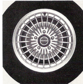
Finned Turbo Cast Aluminum Wheels (UPC N24) Available: All models in gold or silver (14 x 7) (15 x 7 with special performance package only—14 x 7 on Firebird with handling package)
